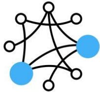
Consortium Blockchain
